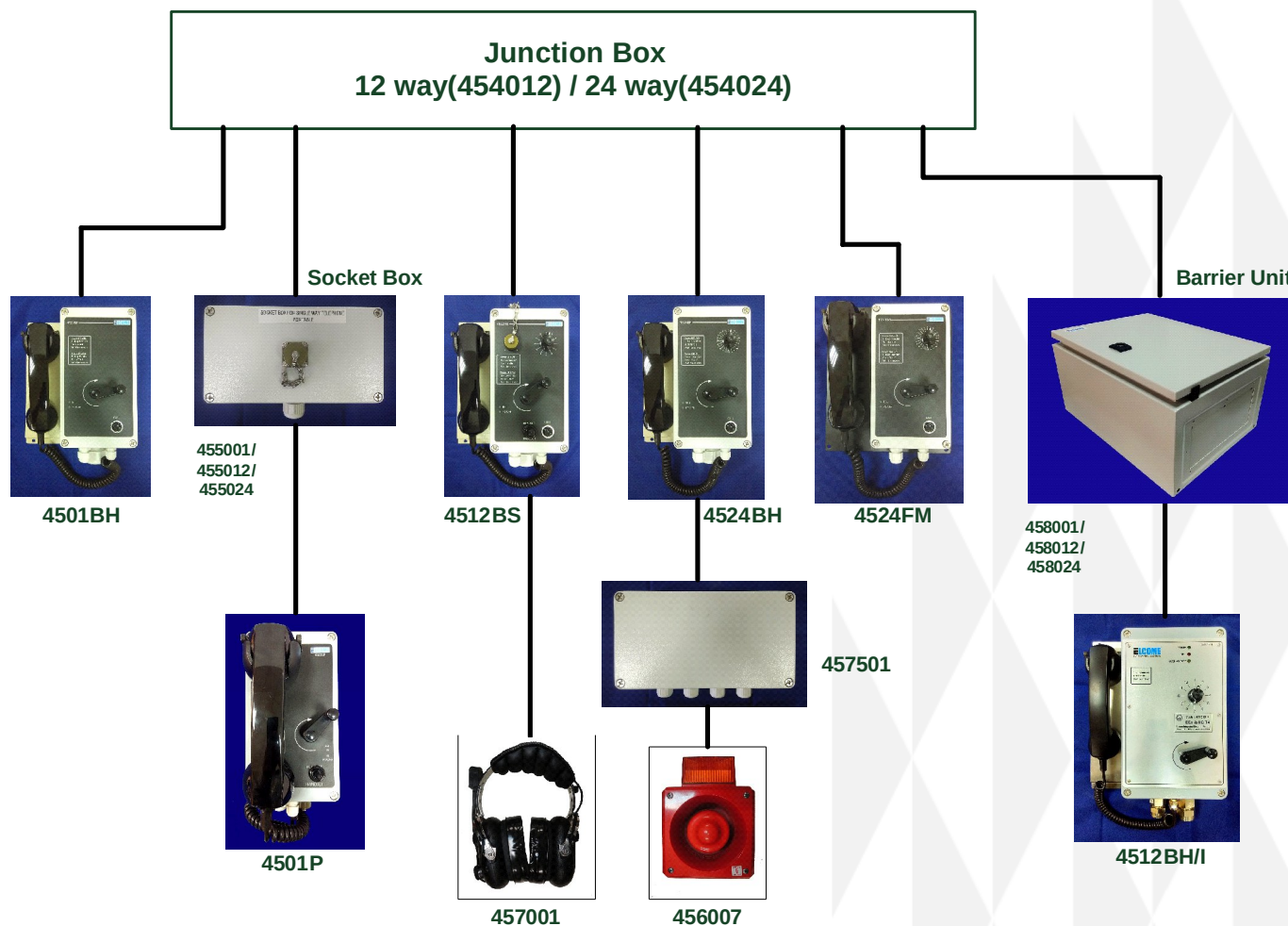
Typical Connection Diagram of SPT 4500 System
